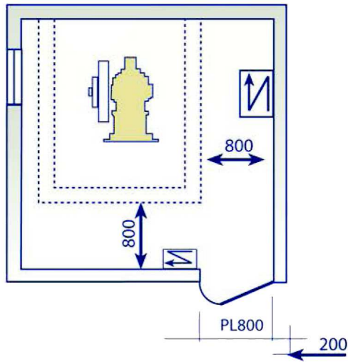
PIANTA LOCALE MACCHINE MACHINE ROOM'S MAP
